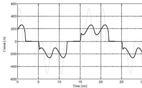
Fig. 2.4 Input current to a drive with DC link reactors.
