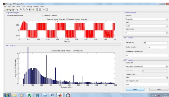
Fig. 3.5 V_{abload} -THD =60.83%
