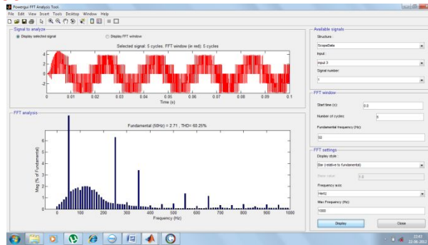
Fig. 3.6 I_{abc} -THD= 60.25%
