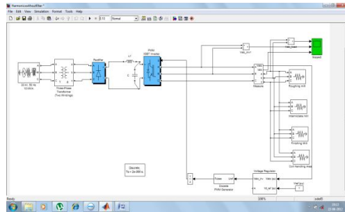
Fig 3.1(a) MATLAB Simulation model of Power System Without Filter
