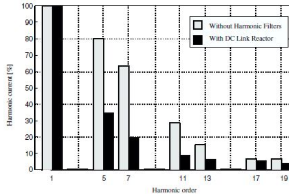
Fig. 2.5: Comparison between the harmonic current spectrum caused by a drive with and without harmonic filters.
