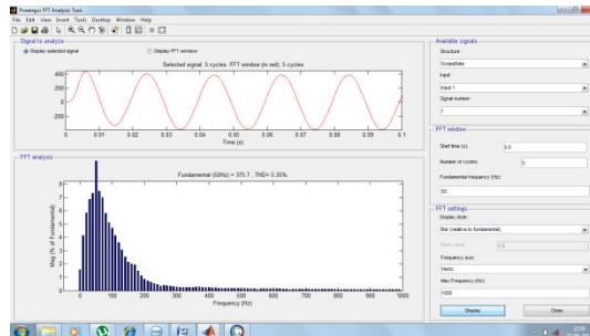
Fig. 3.8 V_{abload} -THD=5.35%
