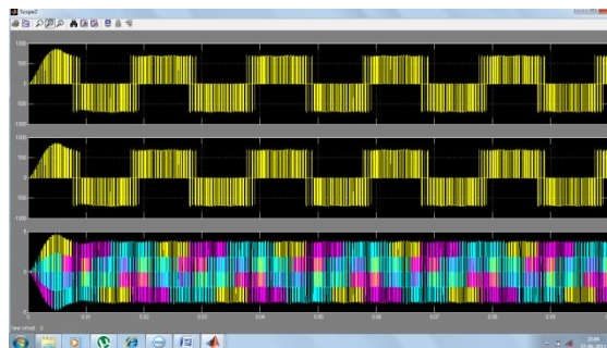
3.2 Waveform of Vinv, Vab load, Iabc (without Harmonics Filter Power system)
