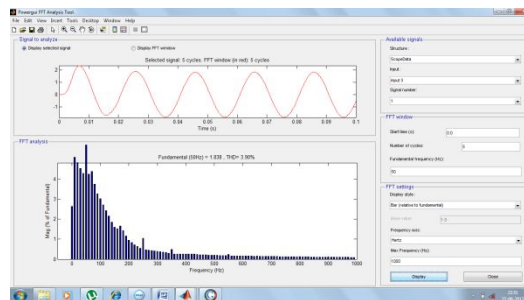
Fig. 3.9 I_{abc} -THD = 3.90%
