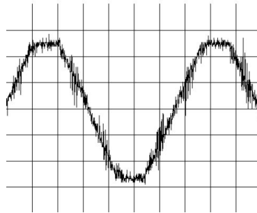
Fig. 2.3 Phase-to-Phase Voltage distortion (“flat topping”) caused by a basic variable frequency drive.
