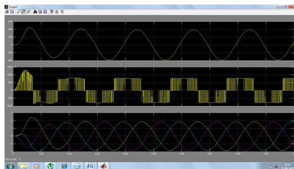
3.3 Waveform of Vinv, Vab load, Iabc (with Harmonics Filter Power system)
