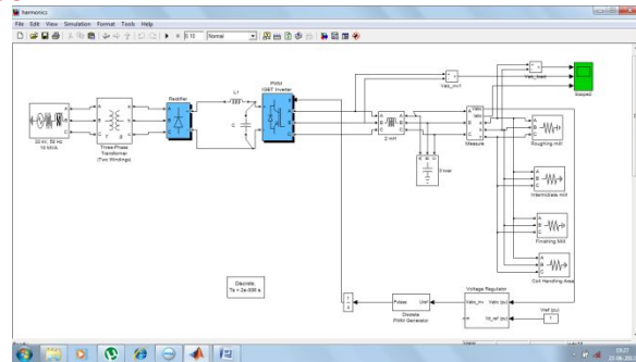
Fig 3.1(b) MATLAB Simulation model of Power System With Filter
