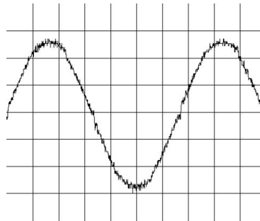
Fig. 2.6 : Input voltage to a drive with DC link reactors.
