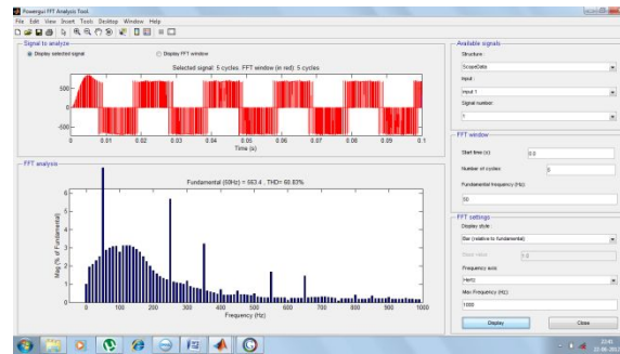
Fig. 3.4 V_{inv} -THD =60.83%
